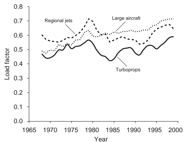
FIGURE 4 Historical trends in load factor for the U.S. large commercial and regional fleets. Reproduced from Lee et al. (2001), with permission.
