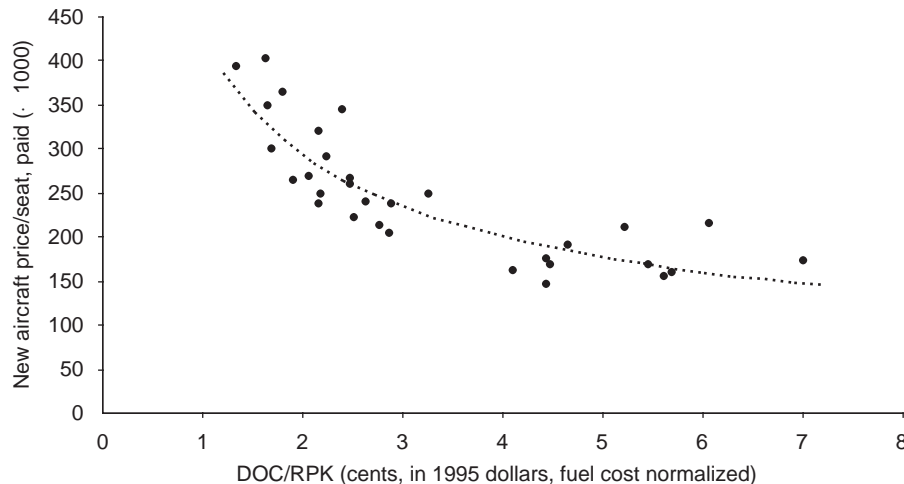
F0030 FIGURE 6 Direct operating cost (DOC) and price relationship. Reported prices are average market values paid in then-year (1995) dollars for new airplanes at the time of purchase. All prices were discounted to 1995 dollars using gross domestic product deflators. RPK, Revenue passenger-kilometers. Reproduced from Lee et al. (2001), with permission.
