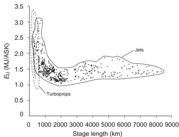
F0015 AU:4 FIGURE 3 Variation of E_U with stage length. ASK, Available seat-kilometers. Reproduced from Lee et al. (2001), with permission.
