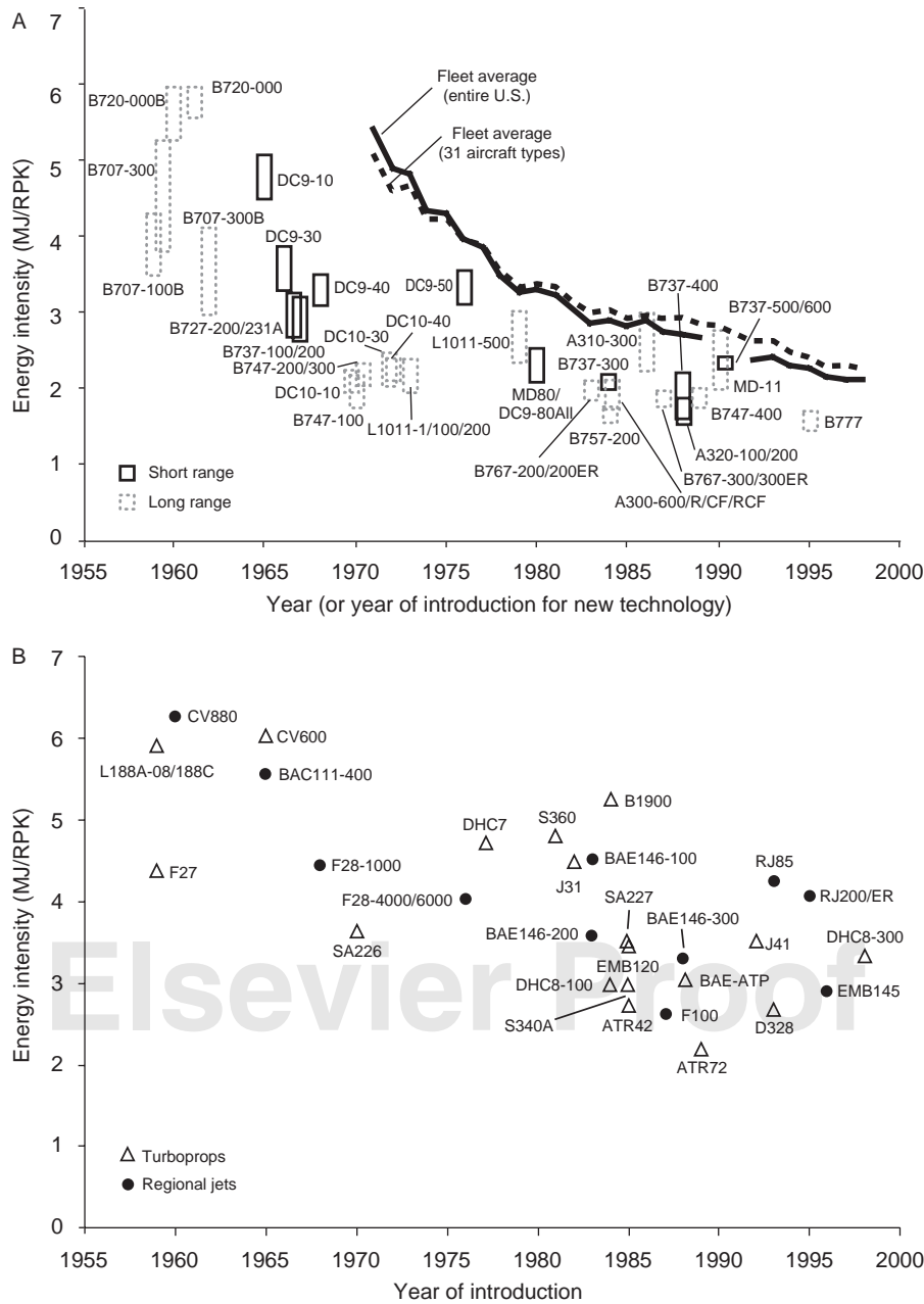
F0010 FIGURE 2 (A) Historical trends in energy intensity of the U.S. large commercial fleets. Individual aircraft E_i based on 1991–1998 operational data with the exception of the B707 and B727, which are based on available operational data prior to 1991. Fleet averages were calculated using a revenue passenger-kilometer (RPK) weighting. Data were not available for the entire U.S. fleet average during 1990 and 1991. (B) Historical trends in energy intensity of the U.S. regional fleets. Reproduced from Lee et al. (2001), with permission.
